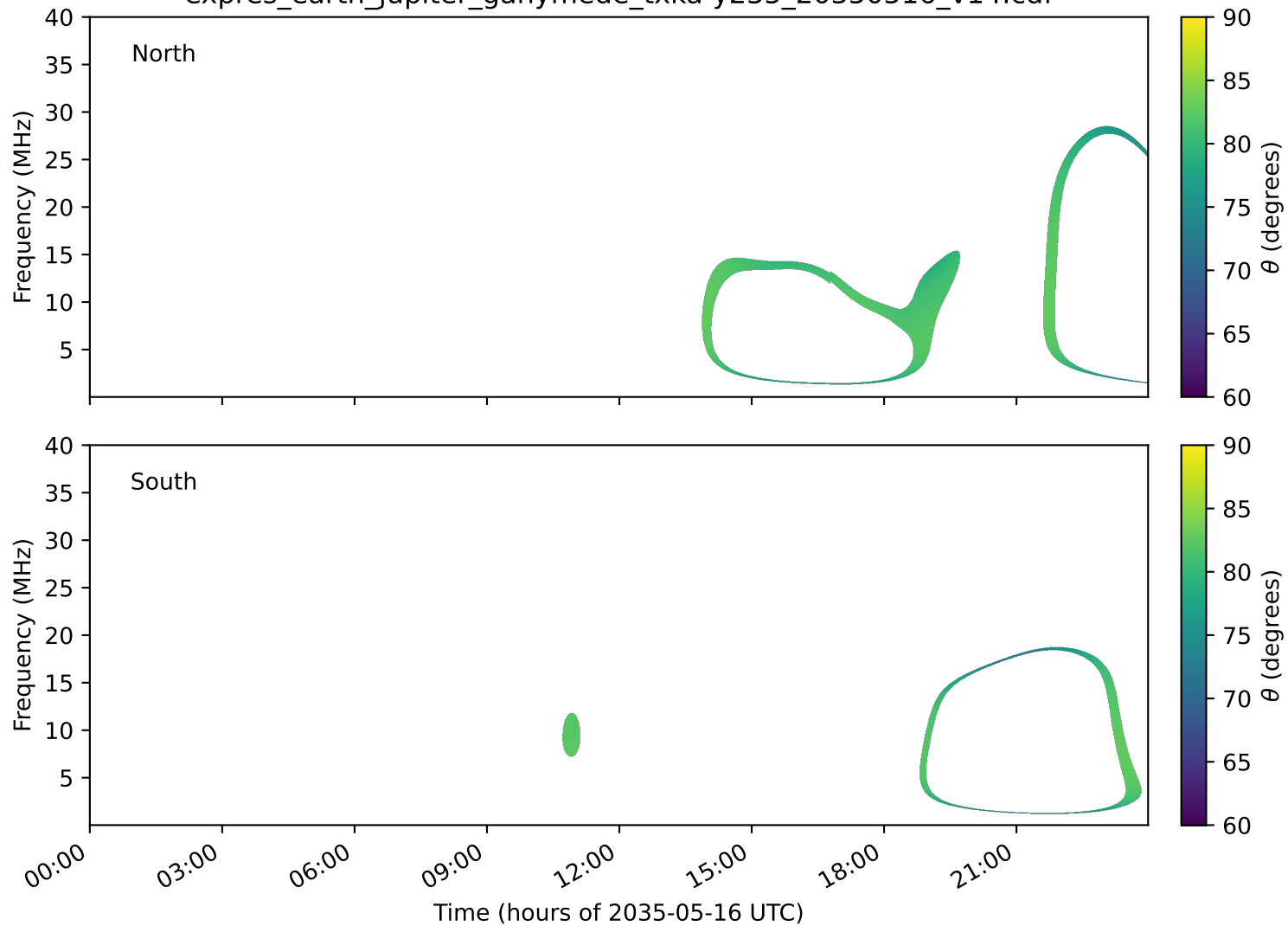
expres_earth_jupiter_ganymede_txka-y235_20350516_v14.cdf
