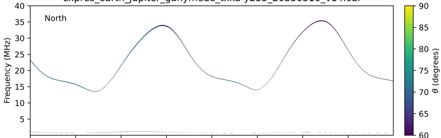
expres_earth_jupiter_ganymede_txka-y235_20350510_v14.cdf
