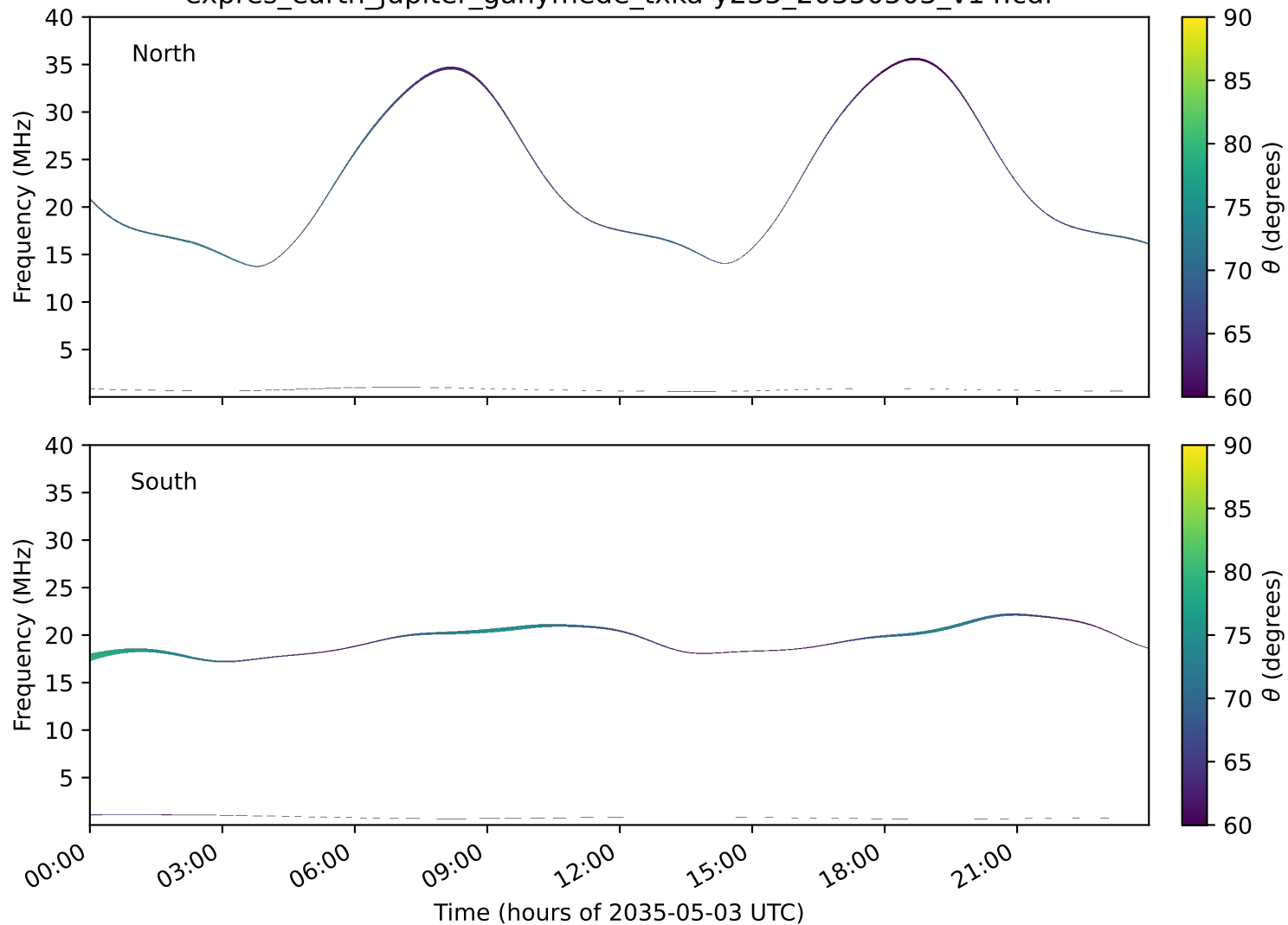
expres_earth_jupiter_ganymede_txka-y235_20350503_v14.cdf
