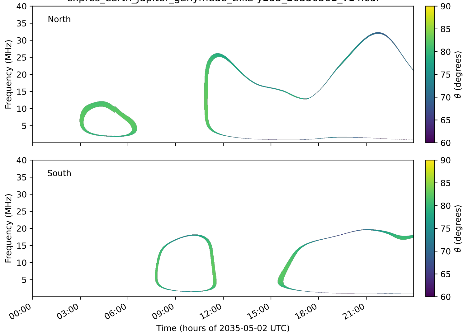
expres_earth_jupiter_ganymede_txka-y235_20350502_v14.cdf
