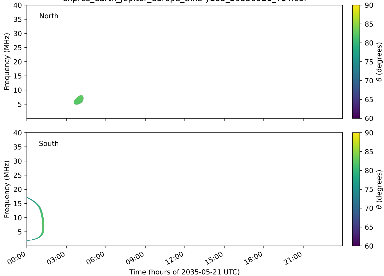
expres_earth_jupiter_europa_txka-y235_20350521_v14.cdf
