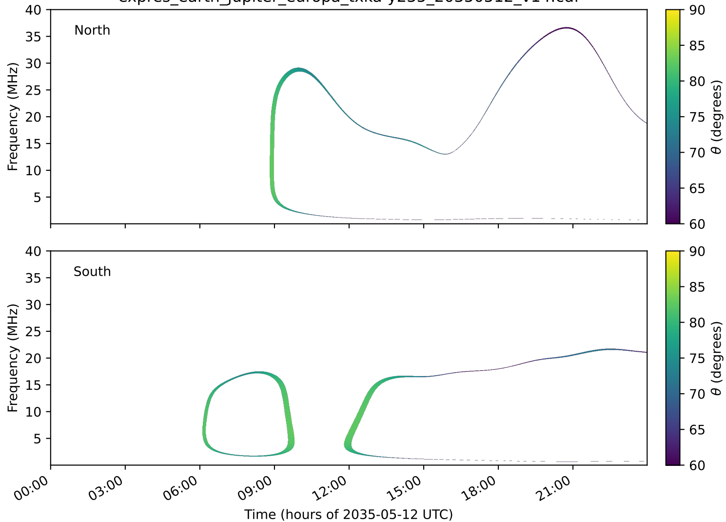
expres_earth_jupiter_europa_txka-y235_20350512_v14.cdf
