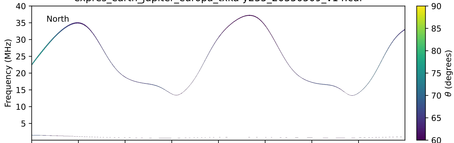
expres_earth_jupiter_europa_txka-y235_20350509_v14.cdf
