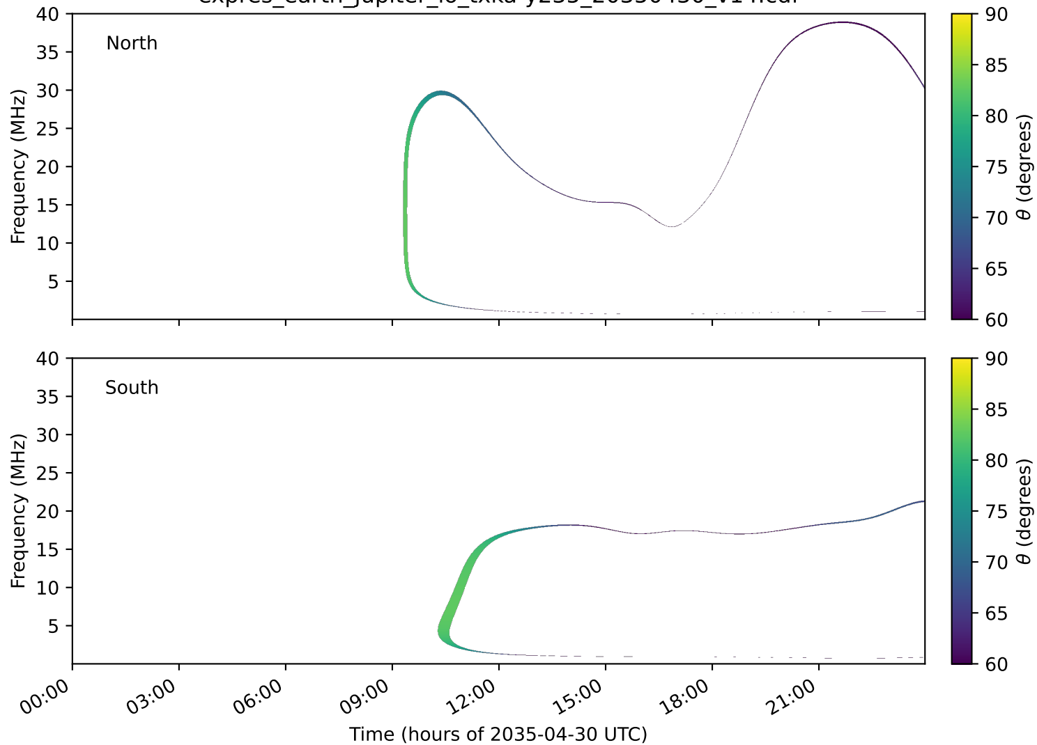
expres_earth_jupiter_io_txka-y235_20350430_v14.cdf
