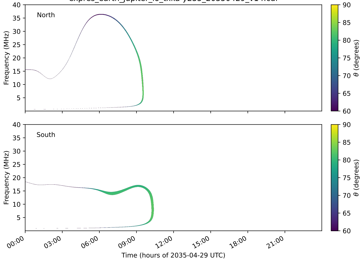
expres_earth_jupiter_io_txka-y235_20350429_v14.cdf
