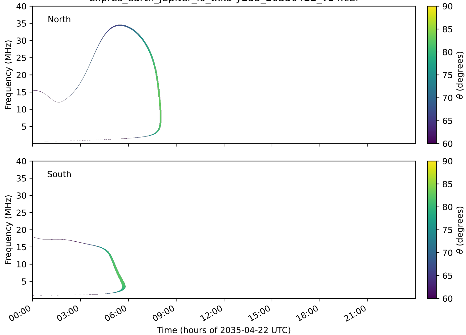
expres_earth_jupiter_io_txka-y235_20350422_v14.cdf
