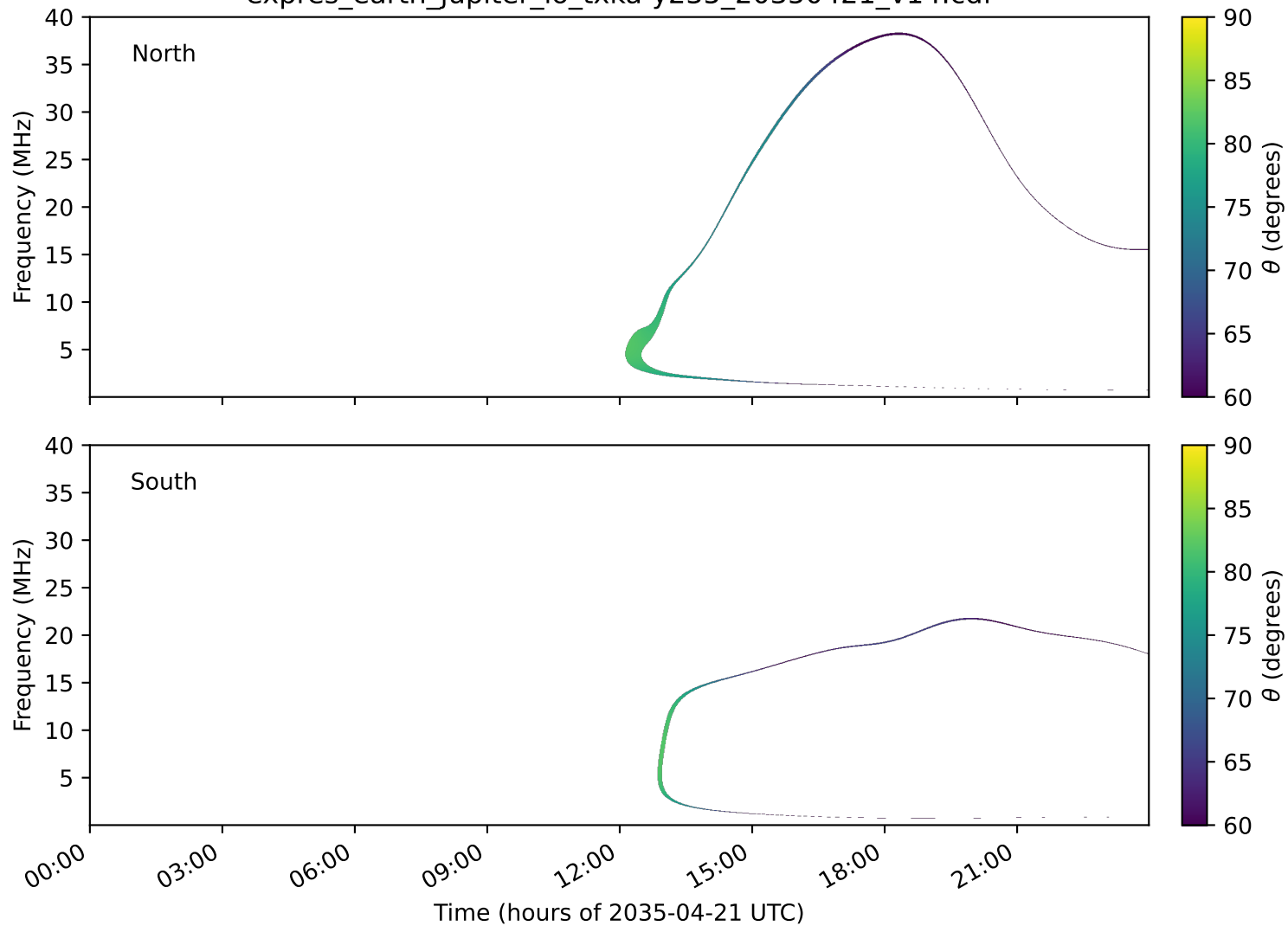
expres_earth_jupiter_io_txka-y235_20350421_v14.cdf
