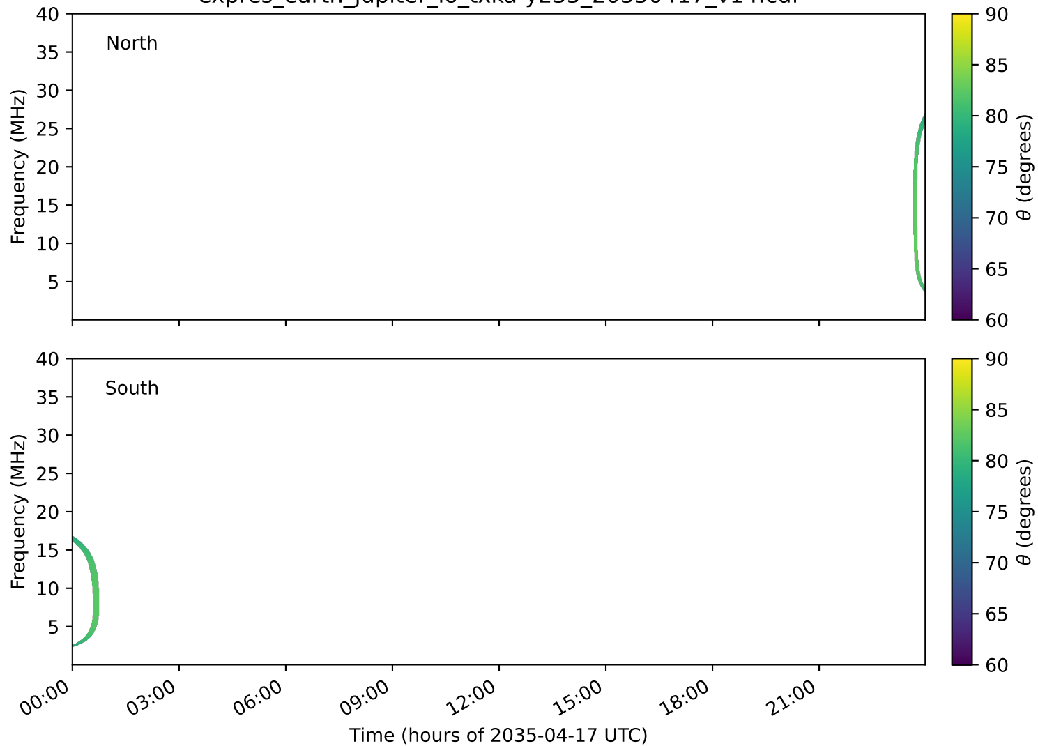
expres_earth_jupiter_io_txka-y235_20350417_v14.cdf
