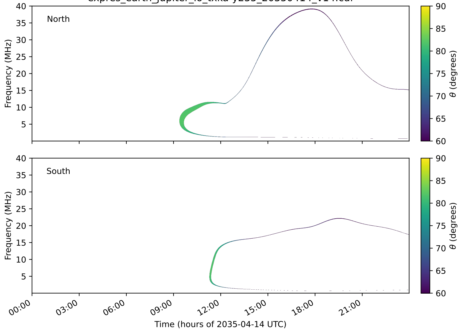
expres_earth_jupiter_io_txka-y235_20350414_v14.cdf
