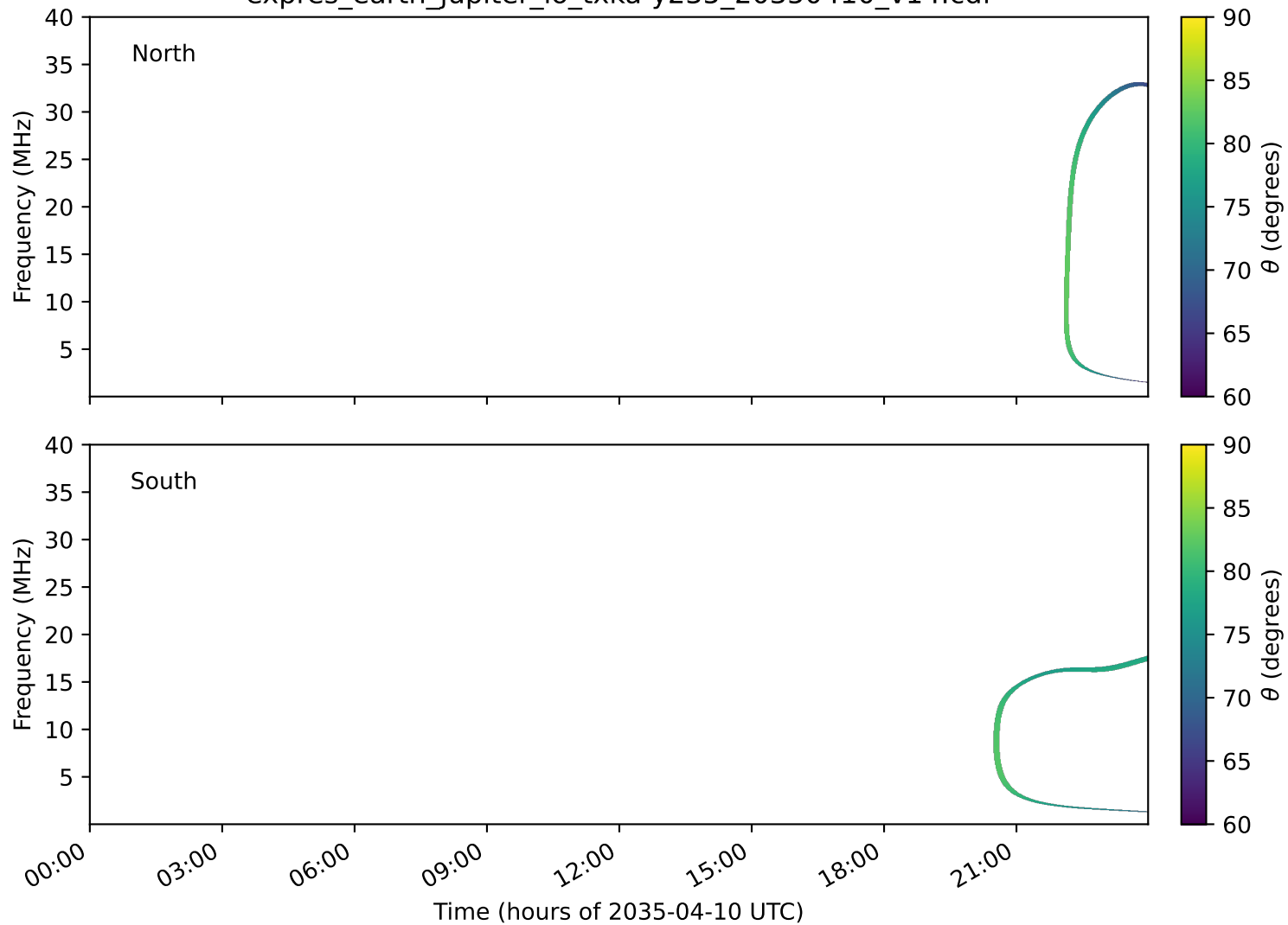
expres_earth_jupiter_io_txka-y235_20350410_v14.cdf
