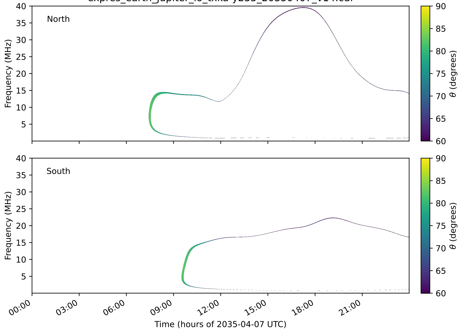
expres_earth_jupiter_io_txka-y235_20350407_v14.cdf
