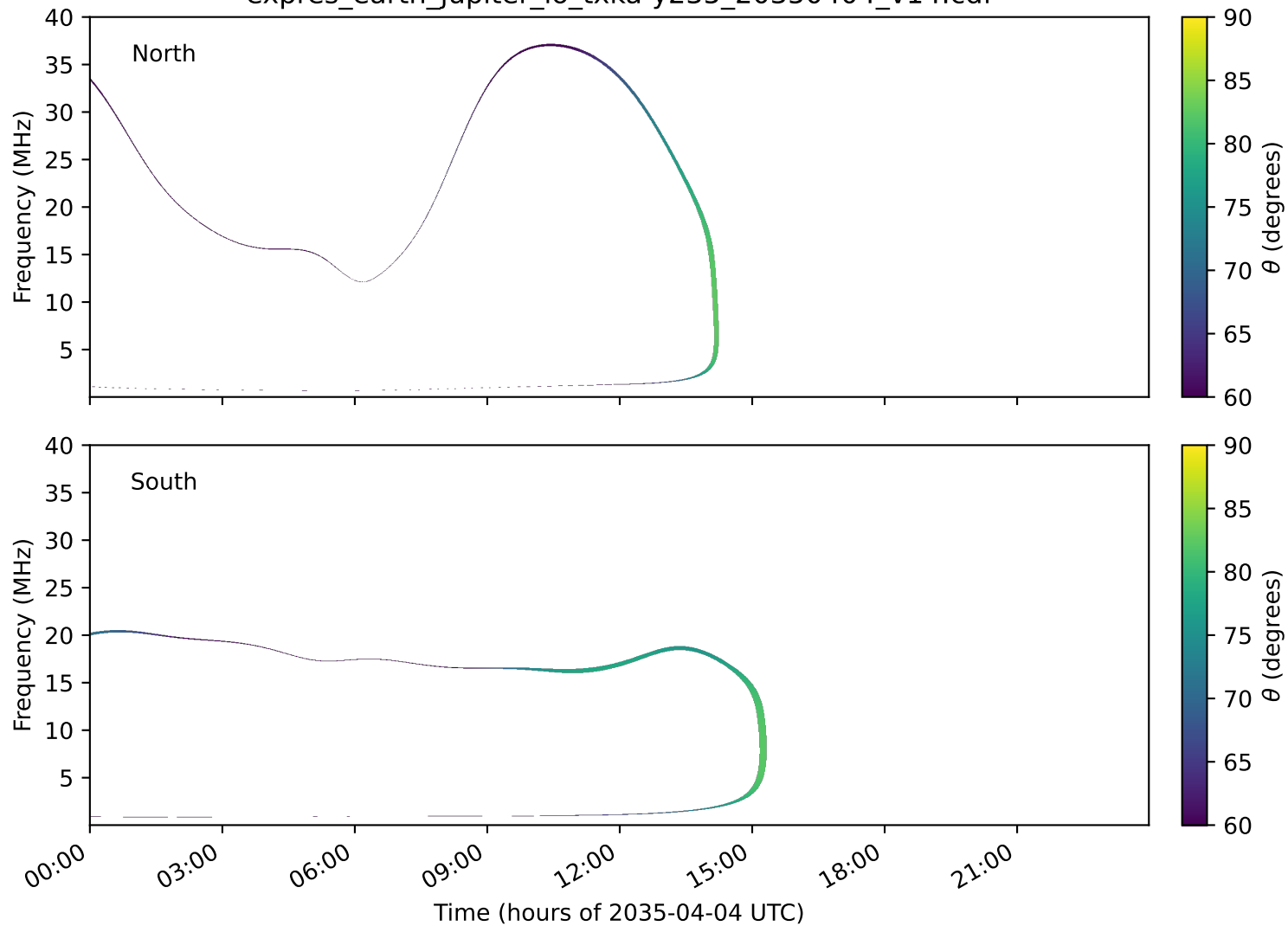
expres_earth_jupiter_io_txka-y235_20350404_v14.cdf
