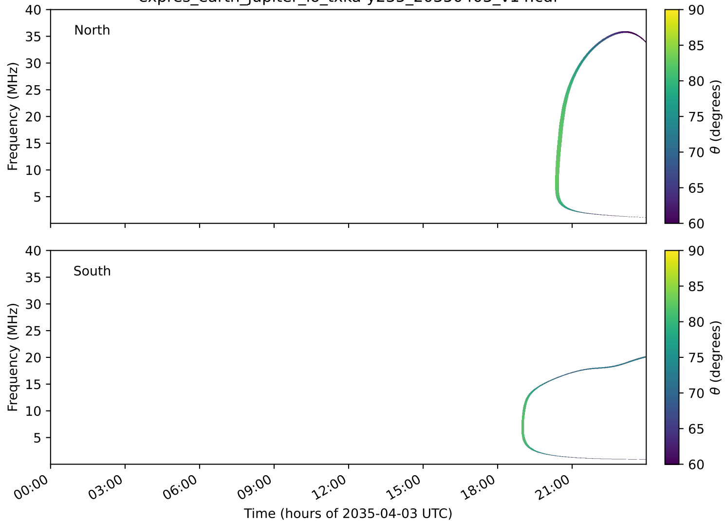
expres_earth_jupiter_io_txka-y235_20350403_v14.cdf
