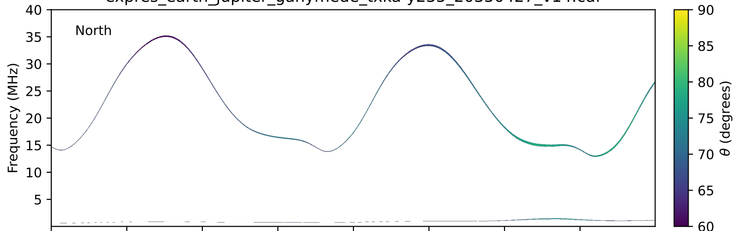
expres_earth_jupiter_ganymede_txka-y235_20350427_v14.cdf
