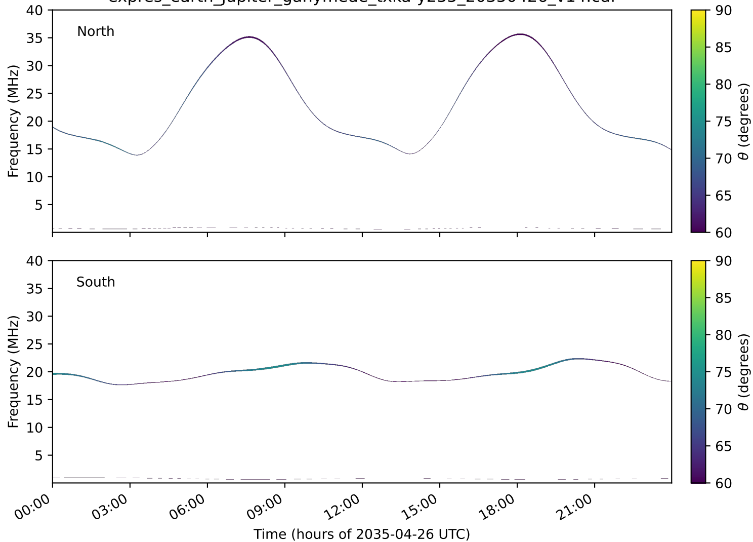
expres_earth_jupiter_ganymede_txka-y235_20350426_v14.cdf
