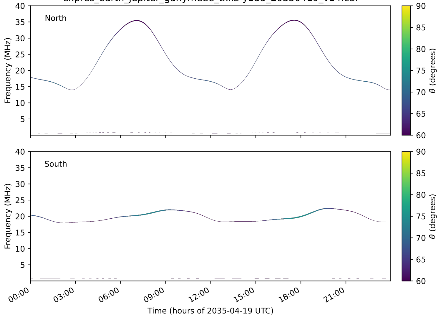
expres_earth_jupiter_ganymede_txka-y235_20350419_v14.cdf
