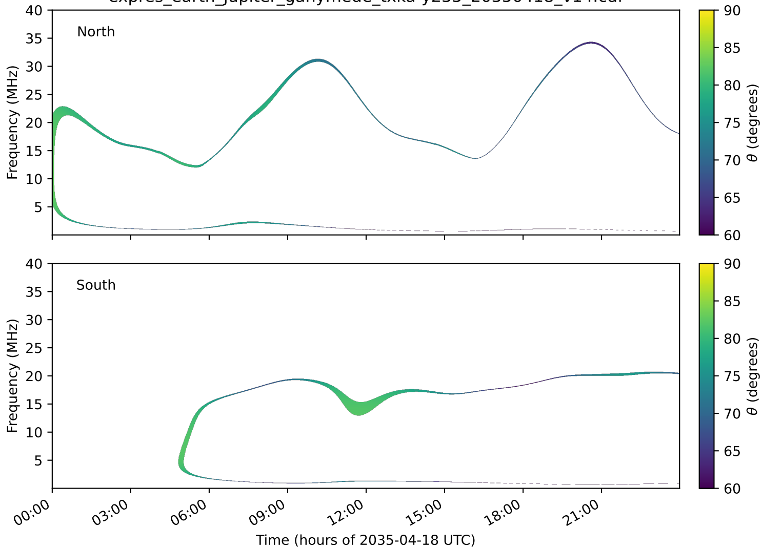
expres_earth_jupiter_ganymede_txka-y235_20350418_v14.cdf
