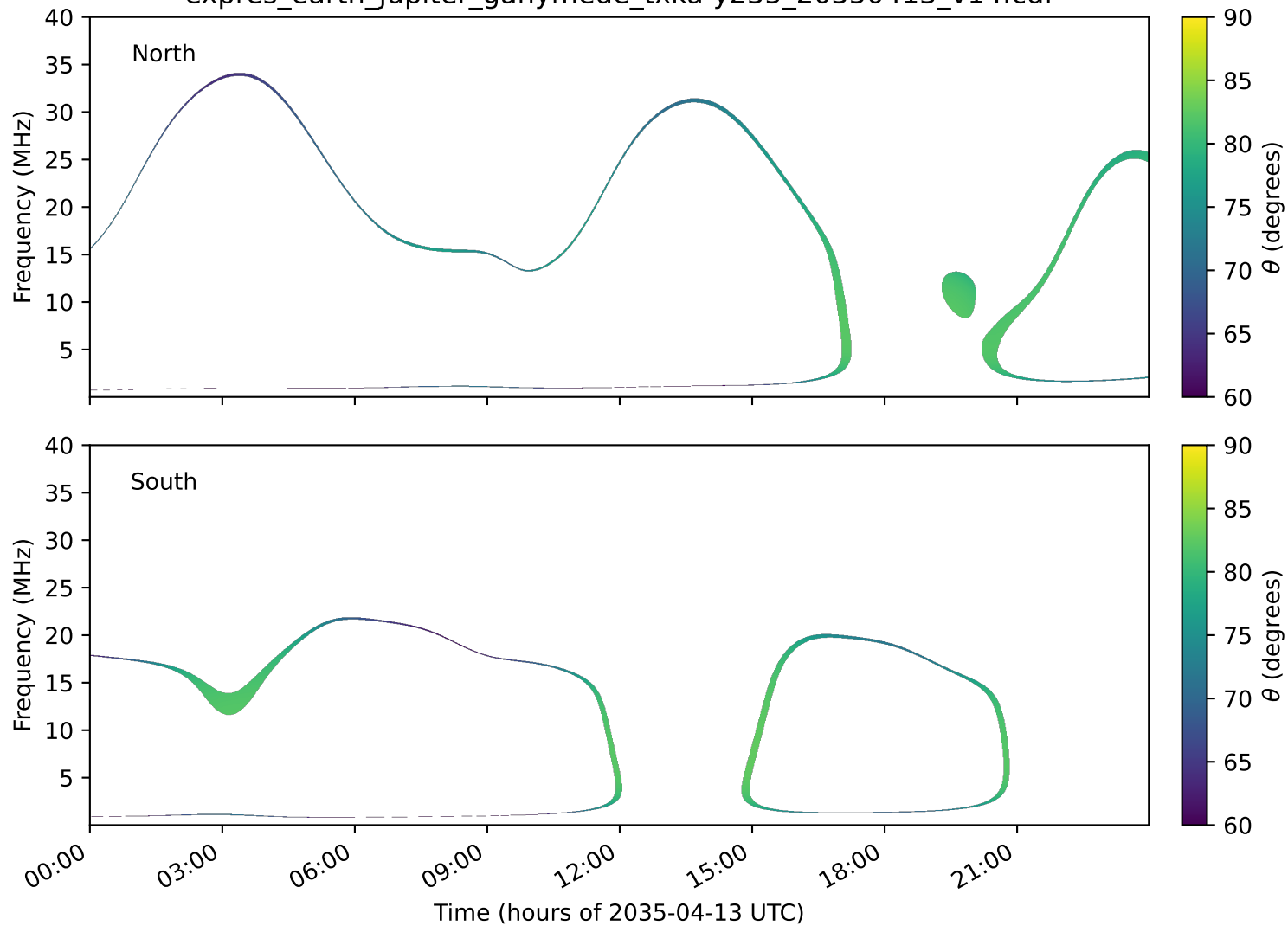
expres_earth_jupiter_ganymede_txka-y235_20350413_v14.cdf
