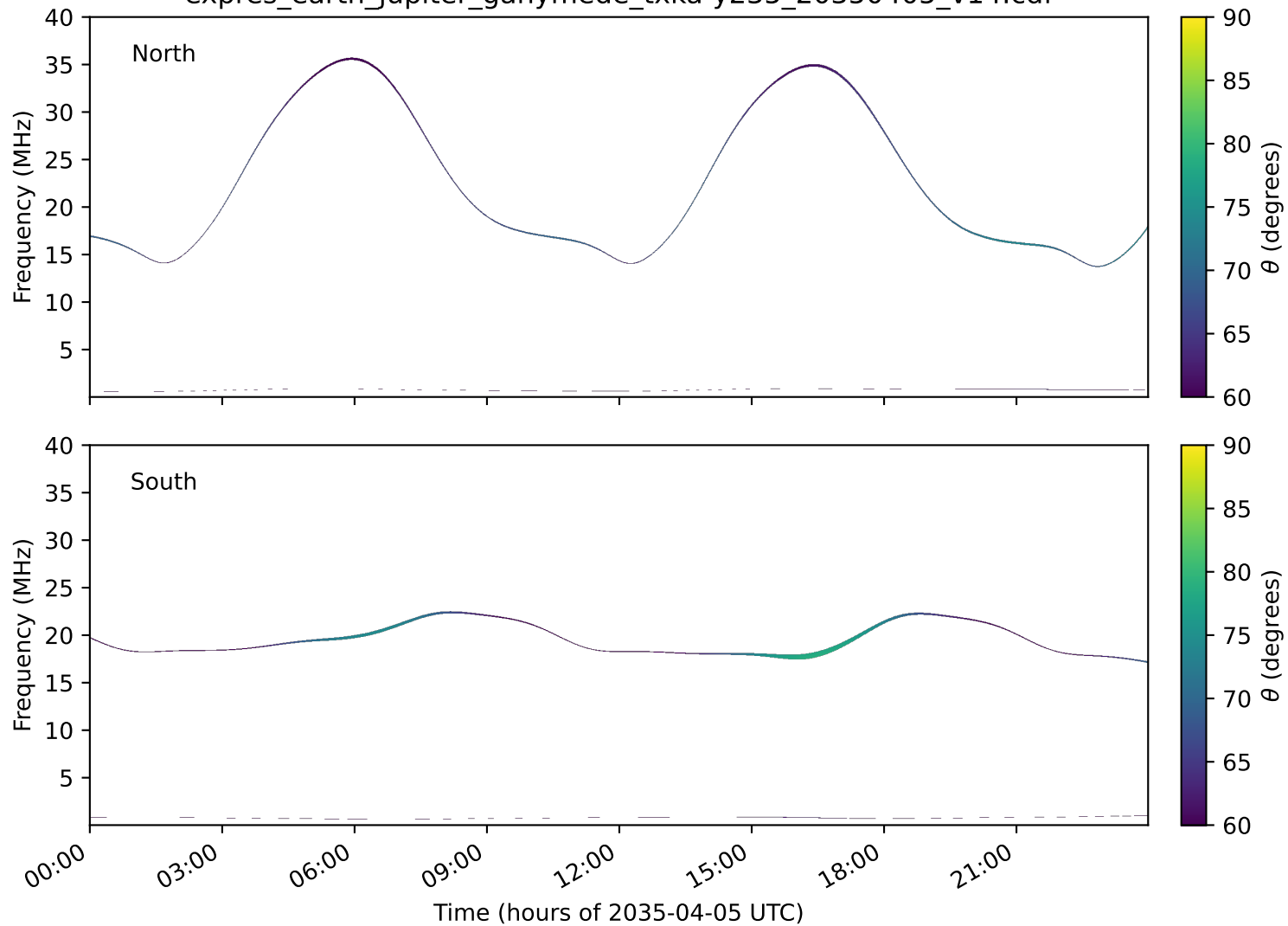
expres_earth_jupiter_ganymede_txka-y235_20350405_v14.cdf
