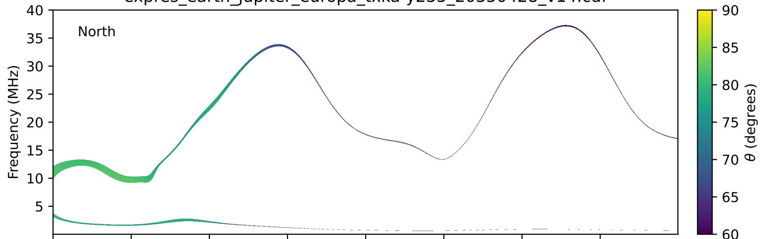
expres_earth_jupiter_europa_txka-y235_20350428_v14.cdf
