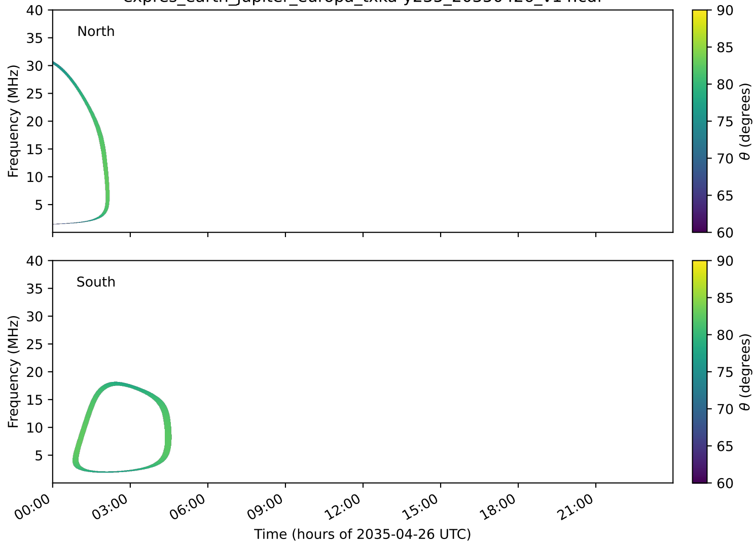
expres_earth_jupiter_europa_txka-y235_20350426_v14.cdf
