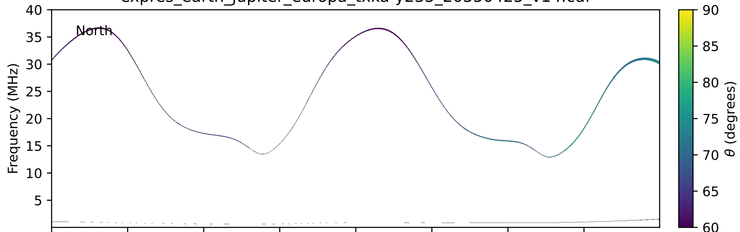
expres_earth_jupiter_europa_txka-y235_20350425_v14.cdf
