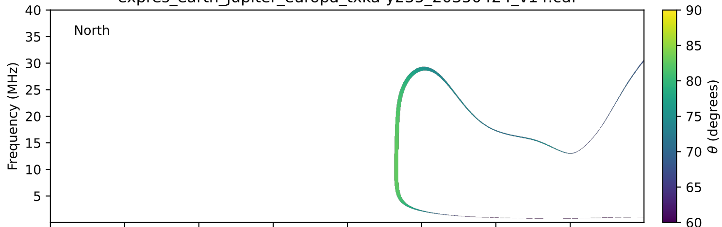
expres_earth_jupiter_europa_txka-y235_20350424_v14.cdf
