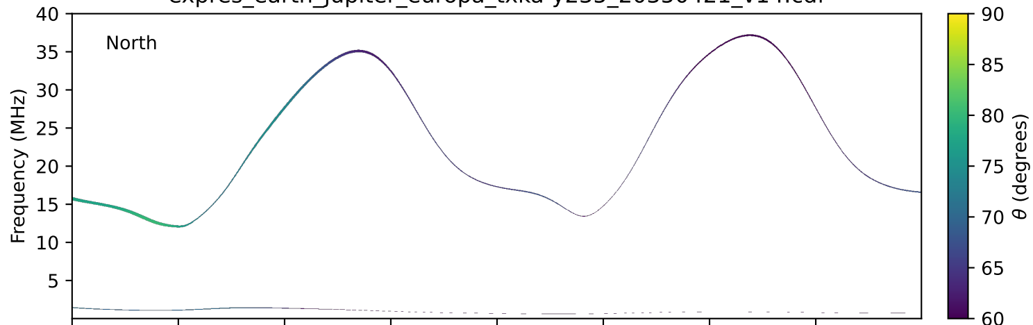
expres_earth_jupiter_europa_txka-y235_20350421_v14.cdf
