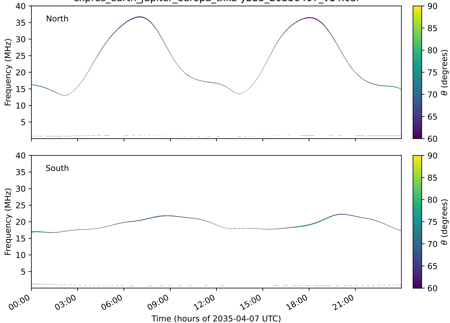
expres_earth_jupiter_europa_txka-y235_20350407_v14.cdf
