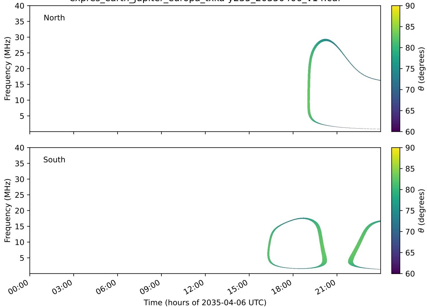
expres_earth_jupiter_europa_txka-y235_20350406_v14.cdf
