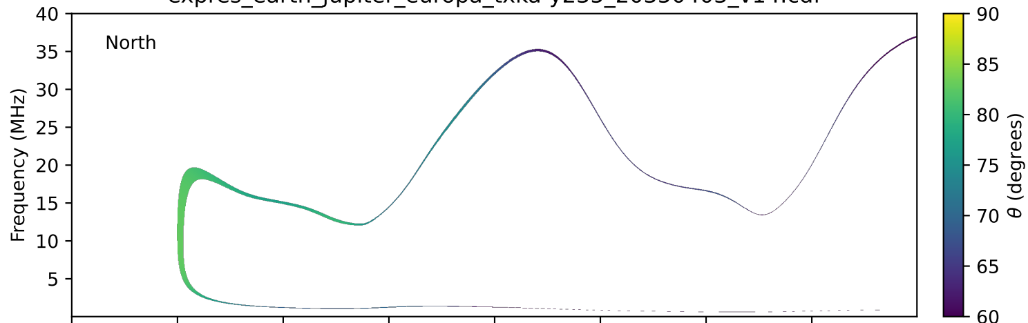
expres_earth_jupiter_europa_txka-y235_20350403_v14.cdf
