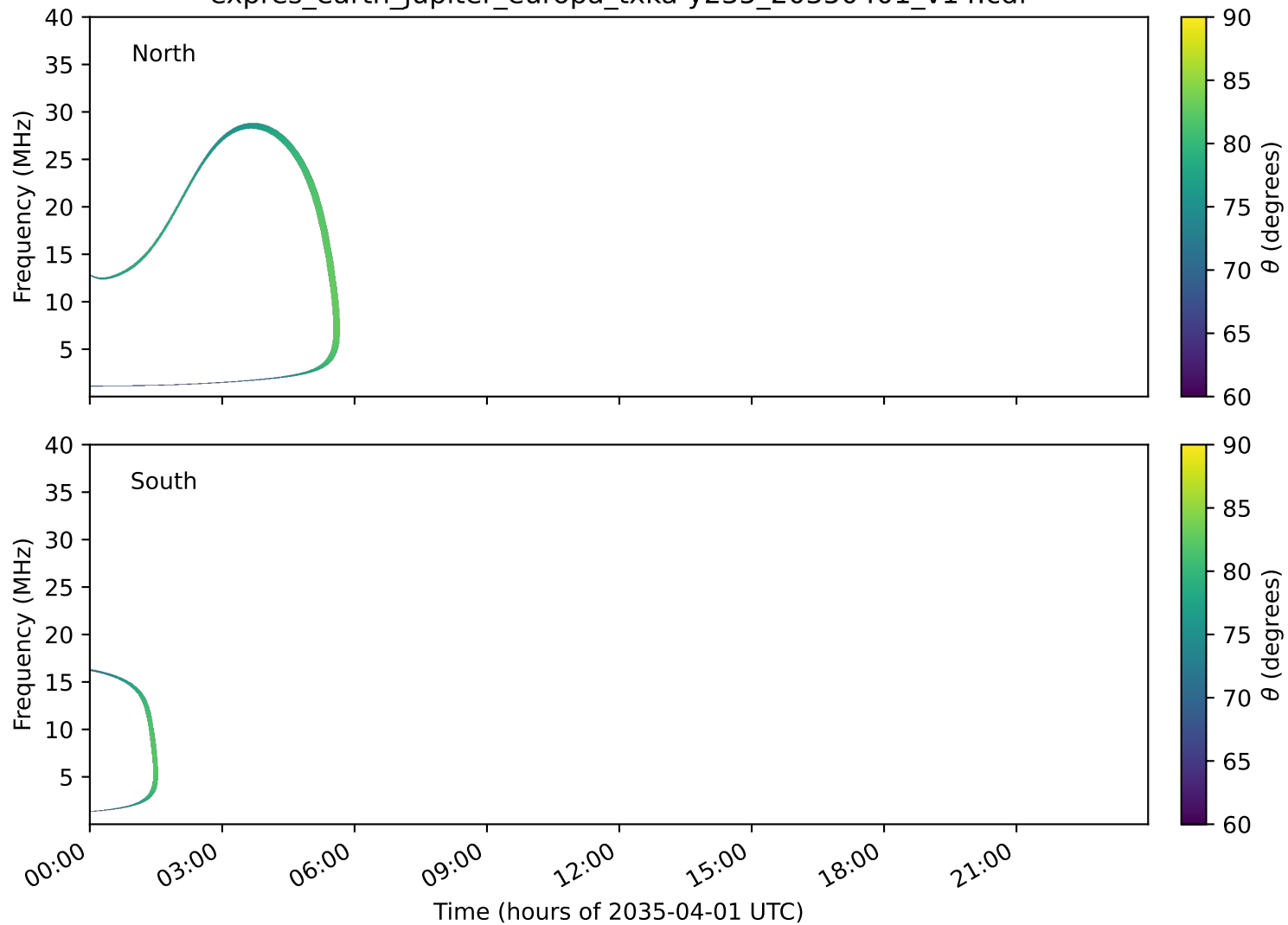
expres_earth_jupiter_europa_txka-y235_20350401_v14.cdf
