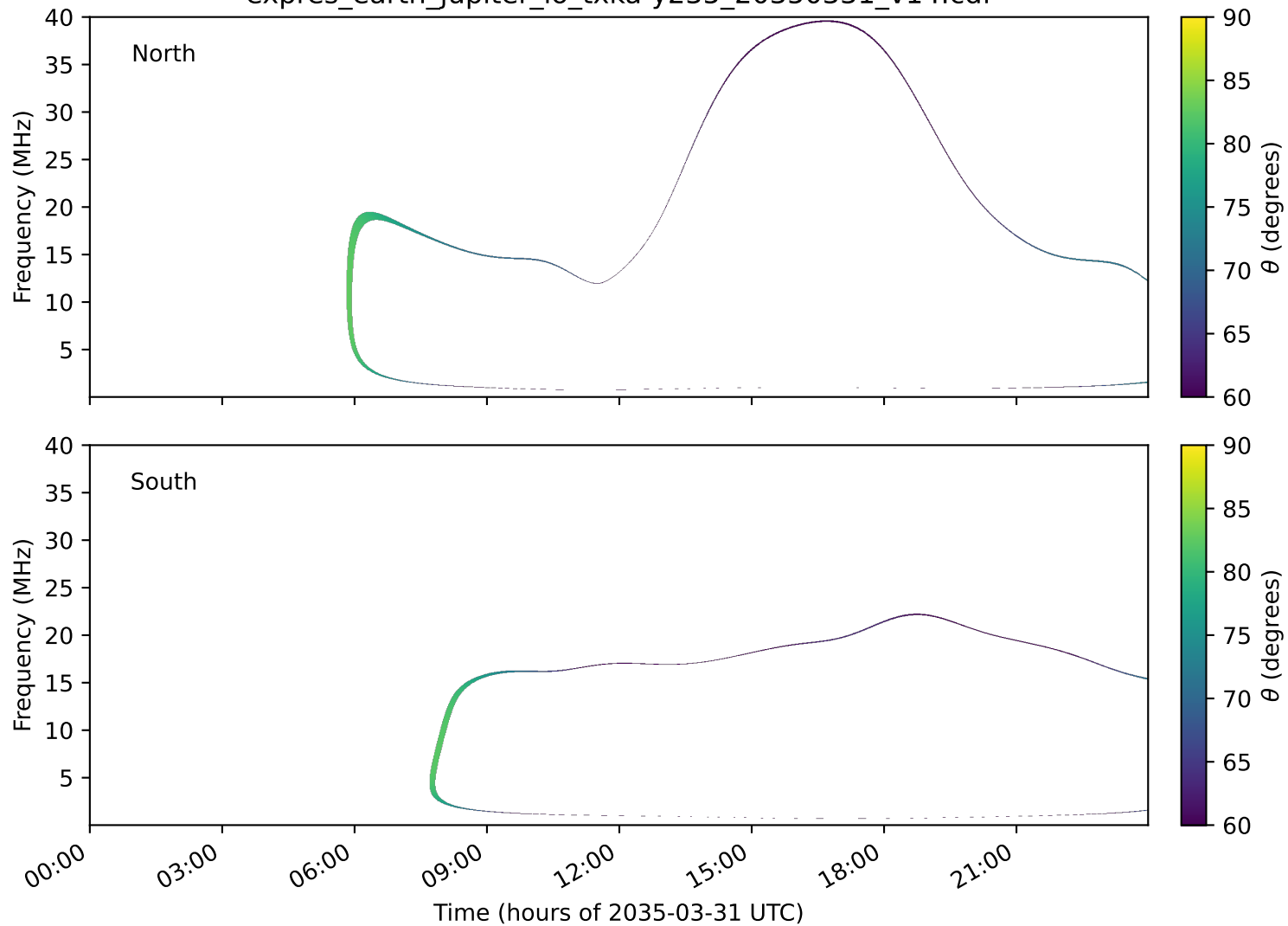
expres_earth_jupiter_io_txka-y235_20350331_v14.cdf
