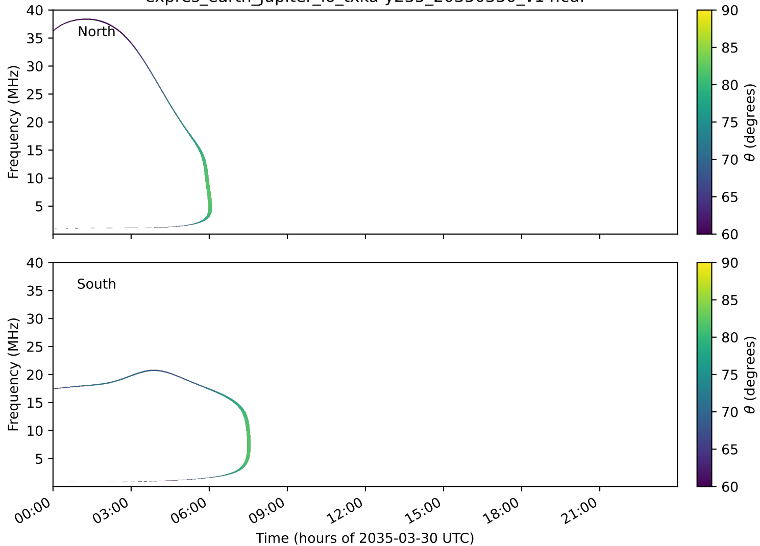
expres_earth_jupiter_io_txka-y235_20350330_v14.cdf
