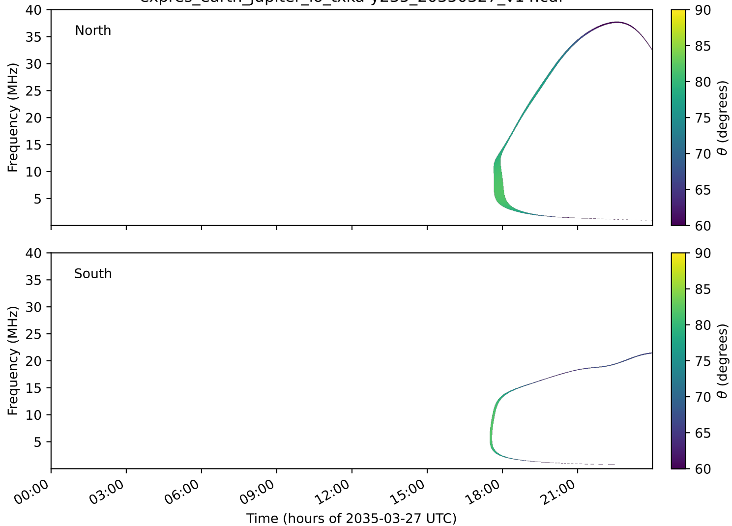
expres_earth_jupiter_io_txka-y235_20350327_v14.cdf
