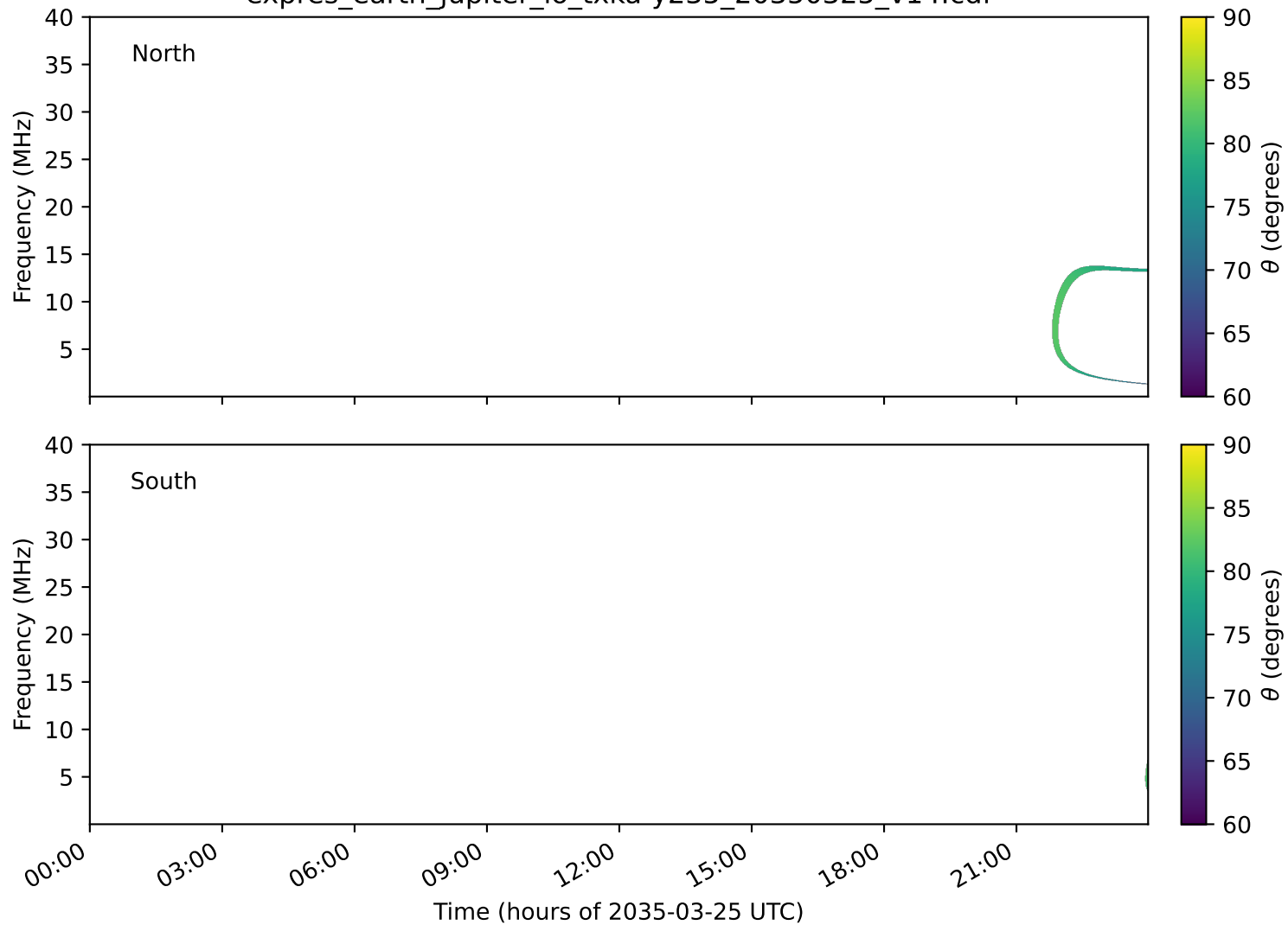
expres_earth_jupiter_io_txka-y235_20350325_v14.cdf
