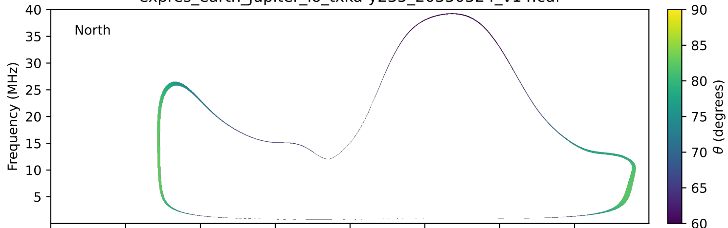
expres_earth_jupiter_io_txka-y235_20350324_v14.cdf
