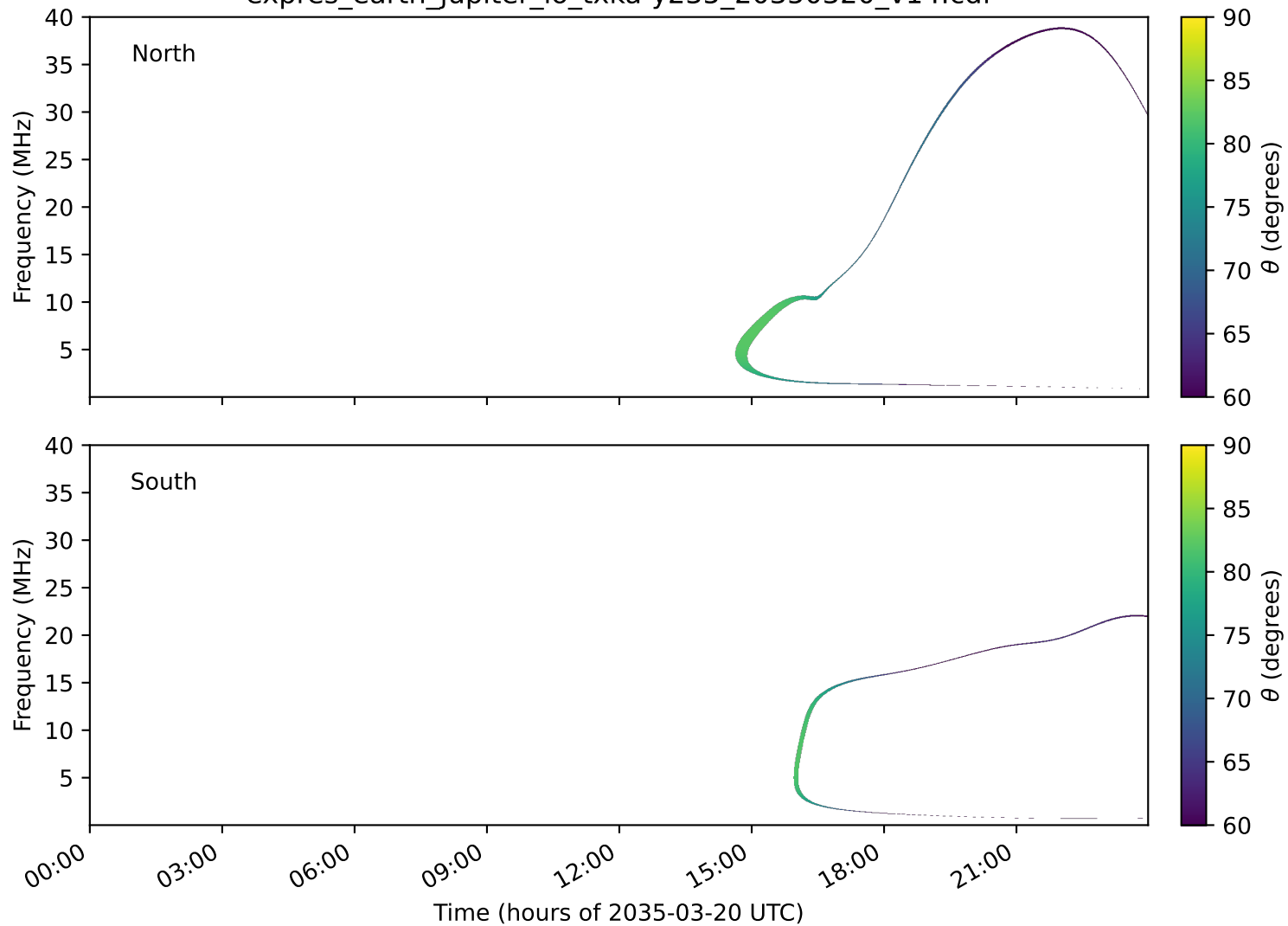
expres_earth_jupiter_io_txka-y235_20350320_v14.cdf
