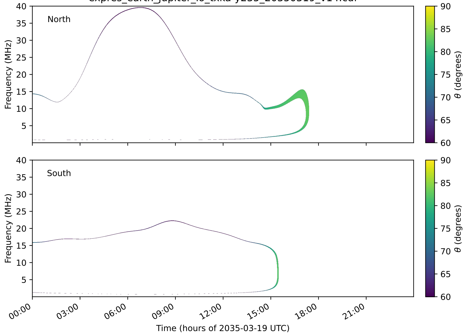
expres_earth_jupiter_io_txka-y235_20350319_v14.cdf
