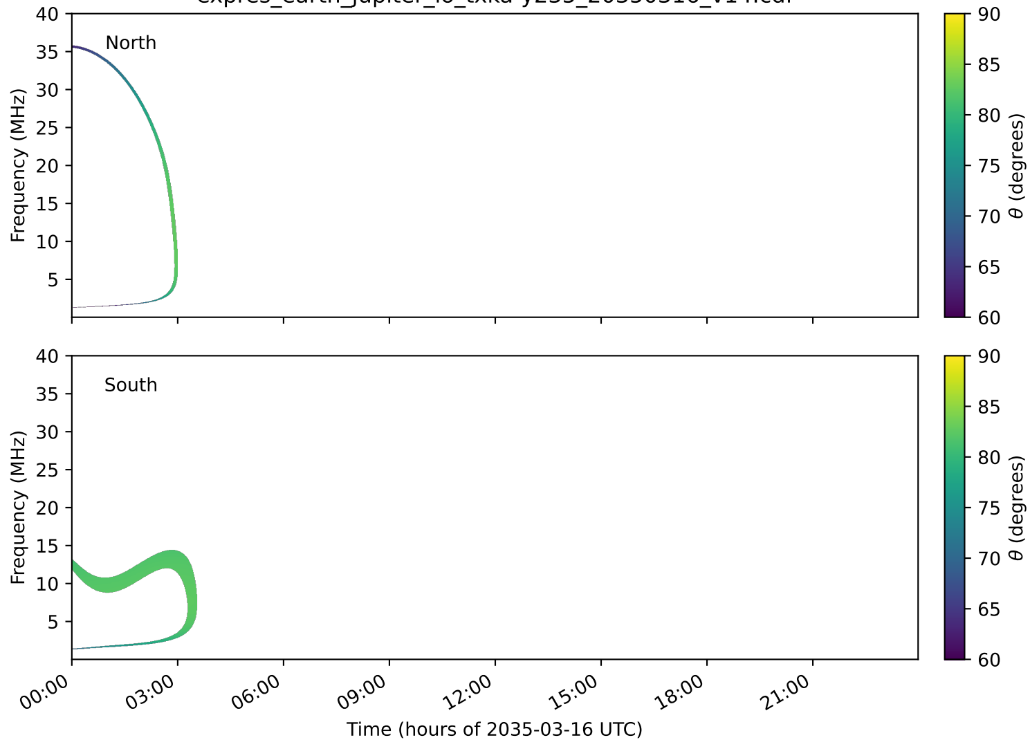
expres_earth_jupiter_io_txka-y235_20350316_v14.cdf
