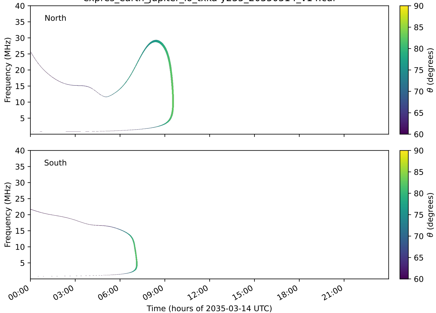
expres_earth_jupiter_io_txka-y235_20350314_v14.cdf
