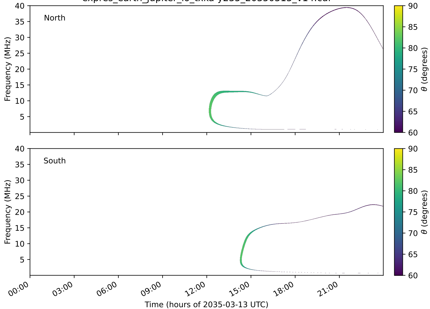
expres_earth_jupiter_io_txka-y235_20350313_v14.cdf
