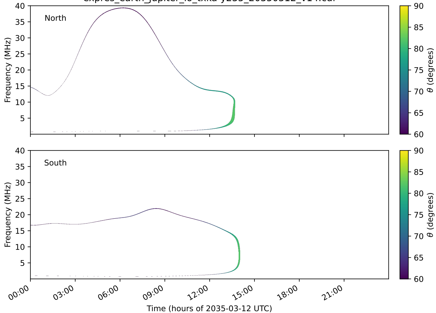
expres_earth_jupiter_io_txka-y235_20350312_v14.cdf
