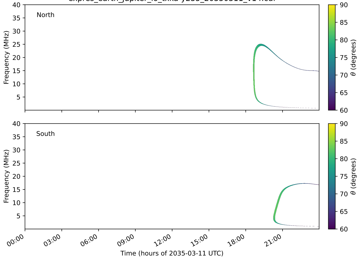
expres_earth_jupiter_io_txka-y235_20350311_v14.cdf
