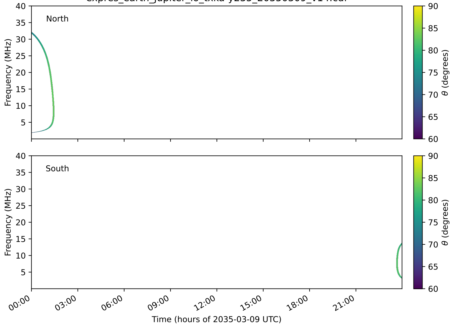
expres_earth_jupiter_io_txka-y235_20350309_v14.cdf
