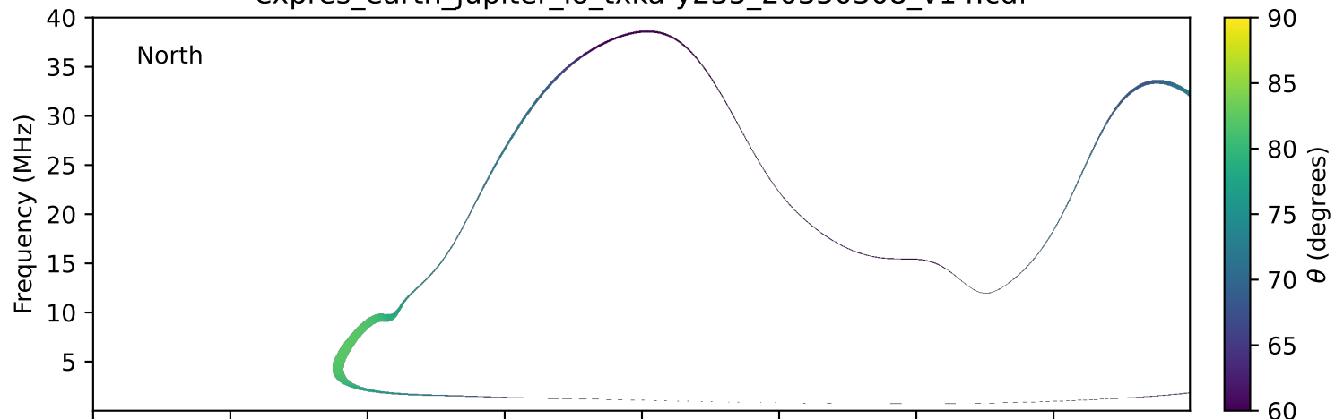
expres_earth_jupiter_io_txka-y235_20350308_v14.cdf
