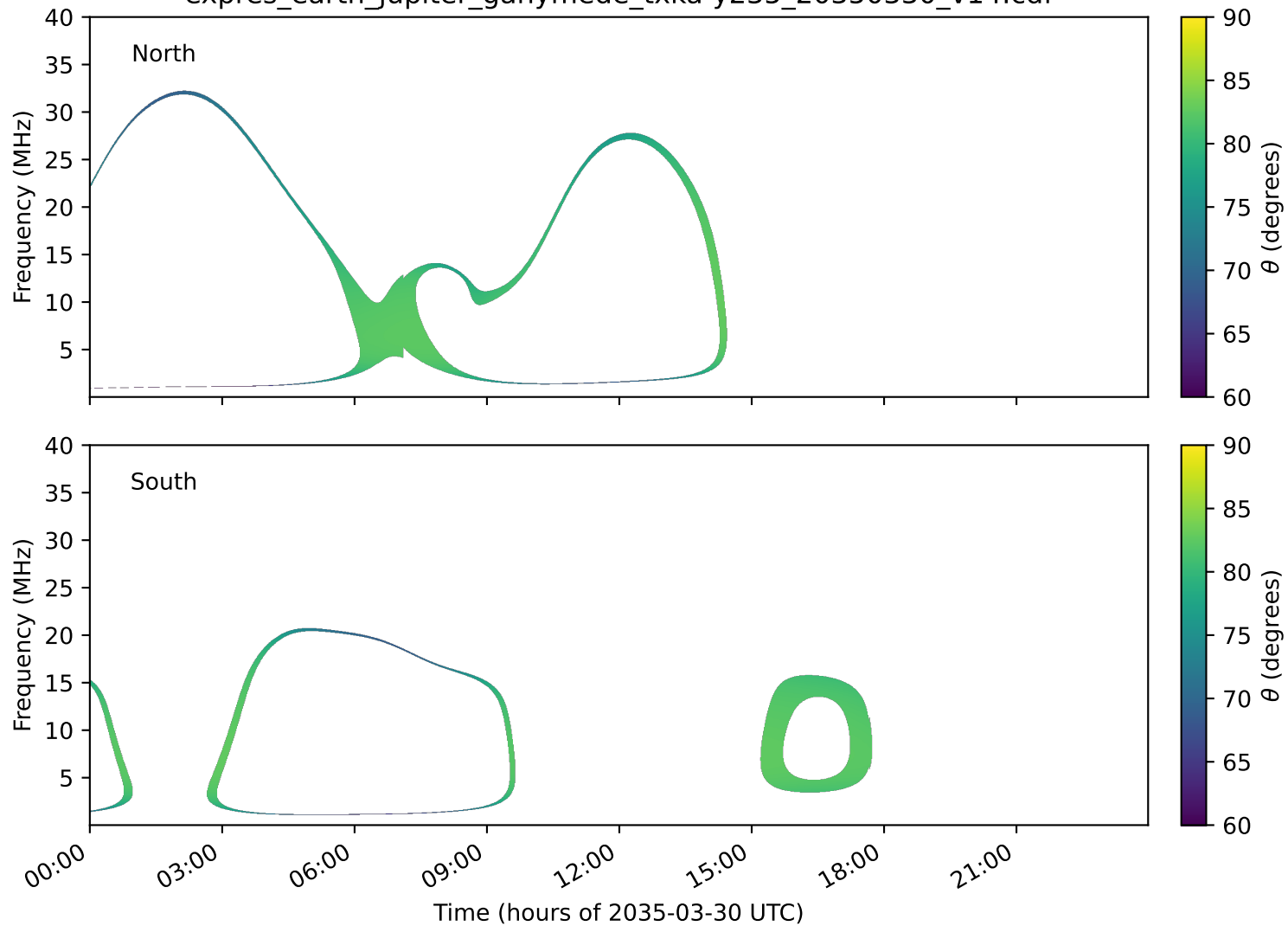
expres_earth_jupiter_ganymede_txka-y235_20350330_v14.cdf
