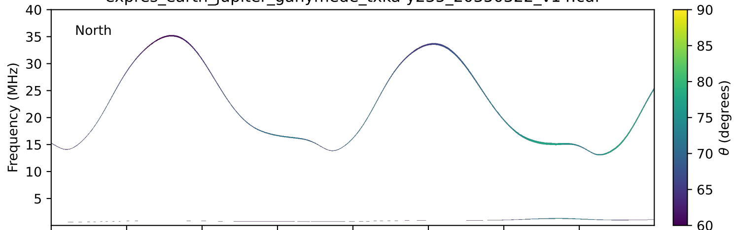
expres_earth_jupiter_ganymede_txka-y235_20350322_v14.cdf
