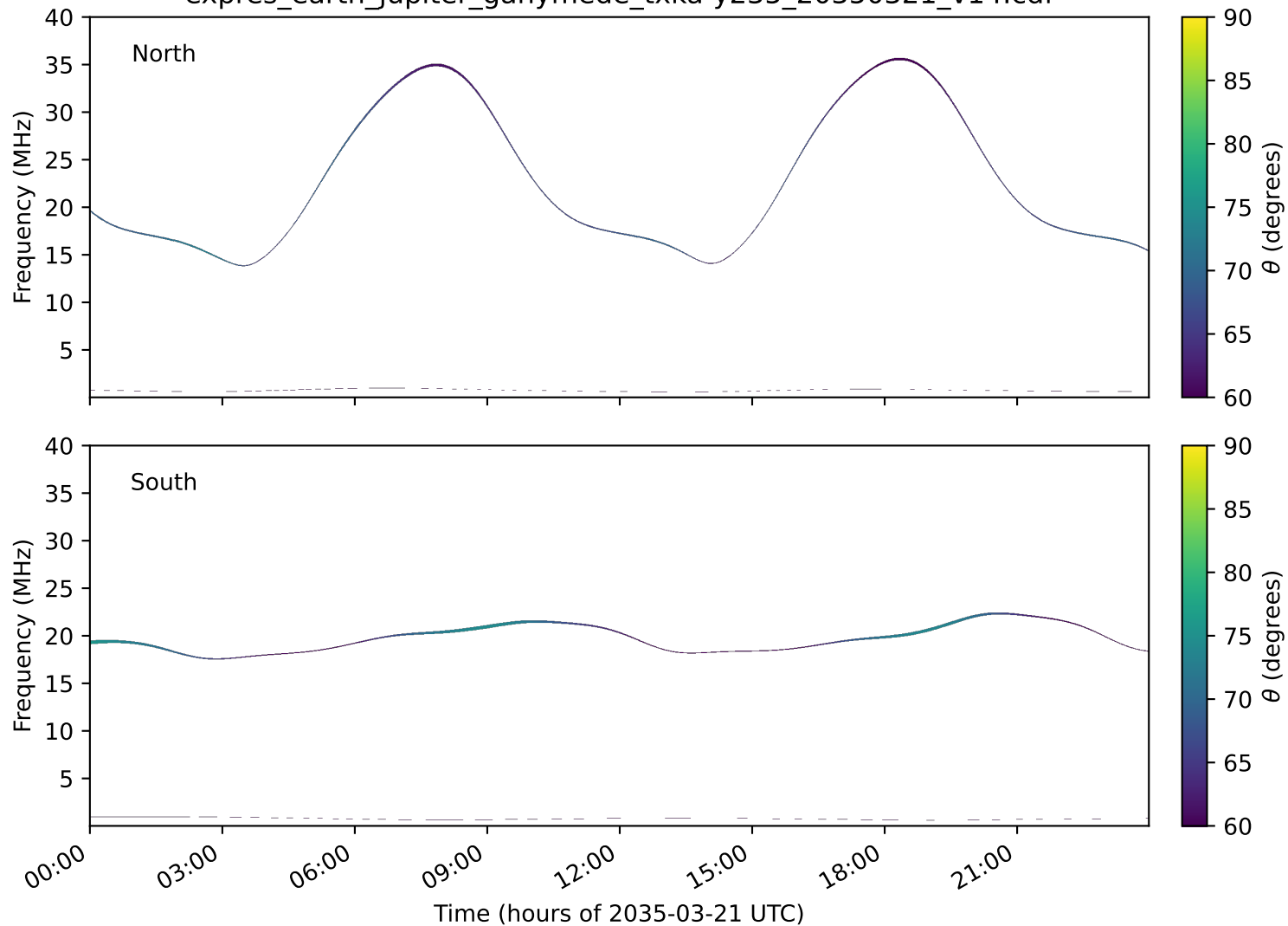
expres_earth_jupiter_ganymede_txka-y235_20350321_v14.cdf
