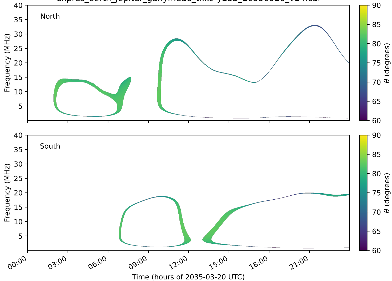
expres_earth_jupiter_ganymede_txka-y235_20350320_v14.cdf
